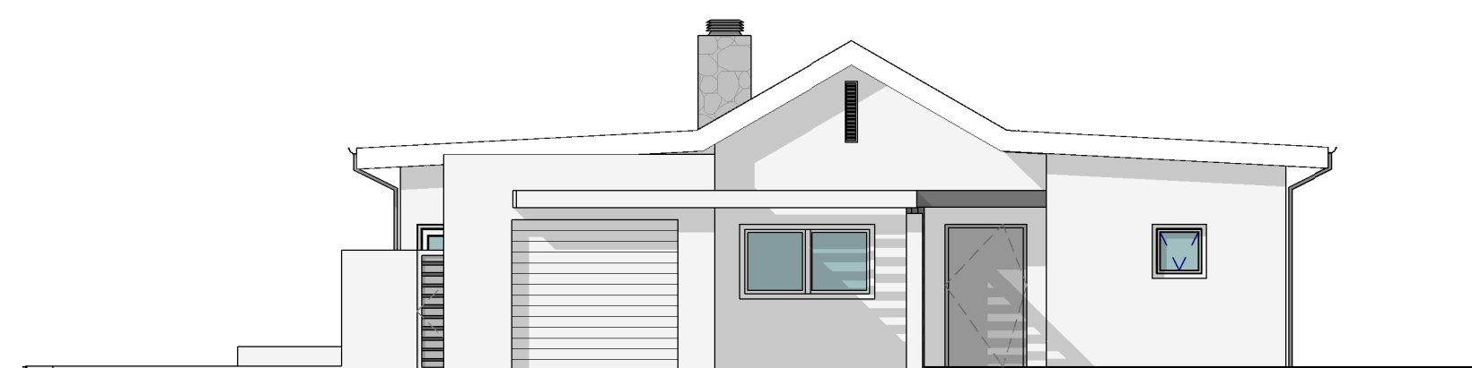
Front Elevation 1 : 100
